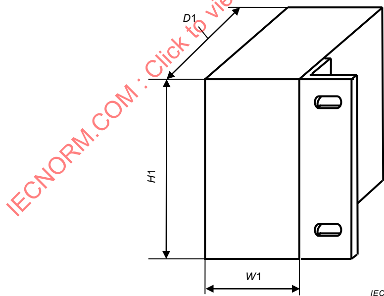
Figure C.3 – Type C: Vertical flange mounting
