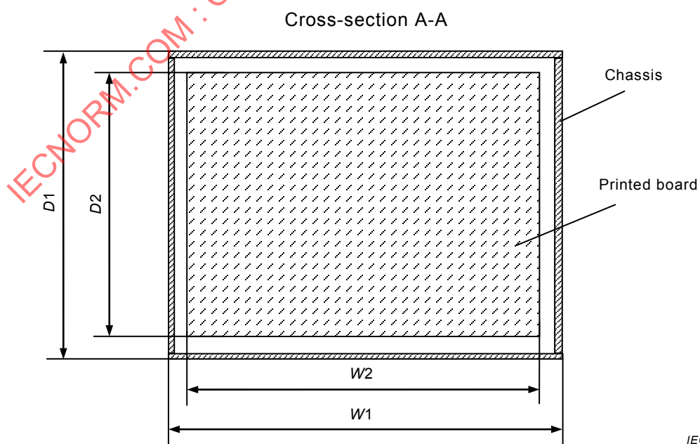
Figure A.2 – Printed board dimensions
