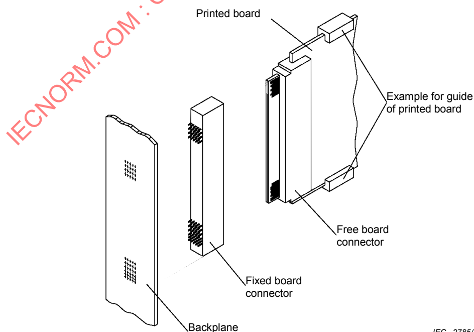
Figure 12 – Fixed board and free board connector – Isometric view
