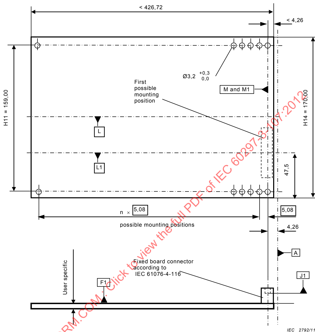
Figure 18b – 4U Backplane dimensions
