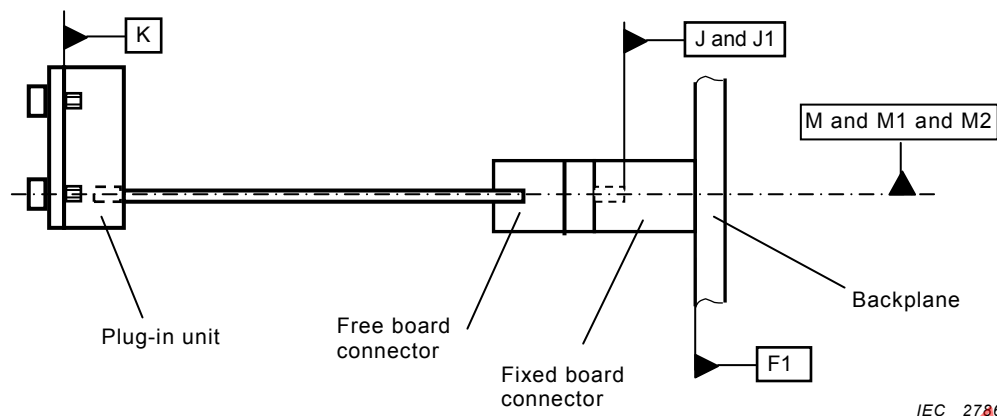
Figure 13 – Two part connector, arrangement overview – Top view
