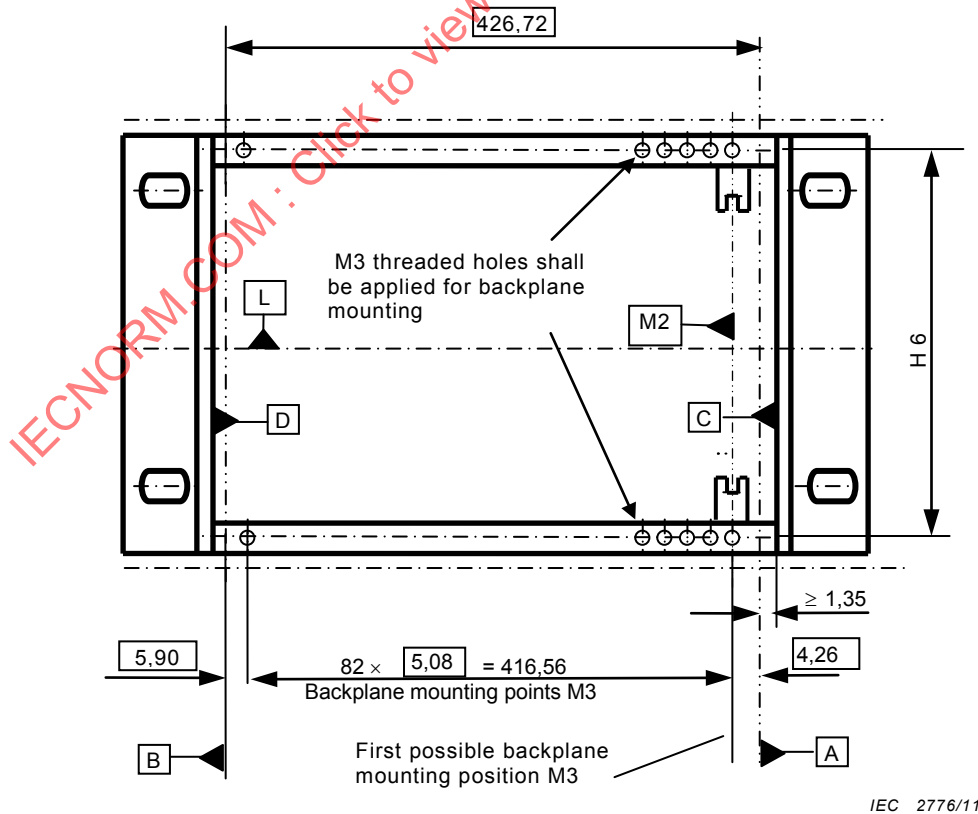
Figure 5 – Subrack dimensions, rear view
