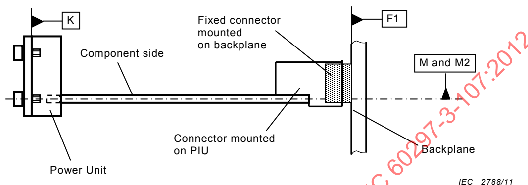
Figure 15 – Two part connector, arrangement overview – Top view
