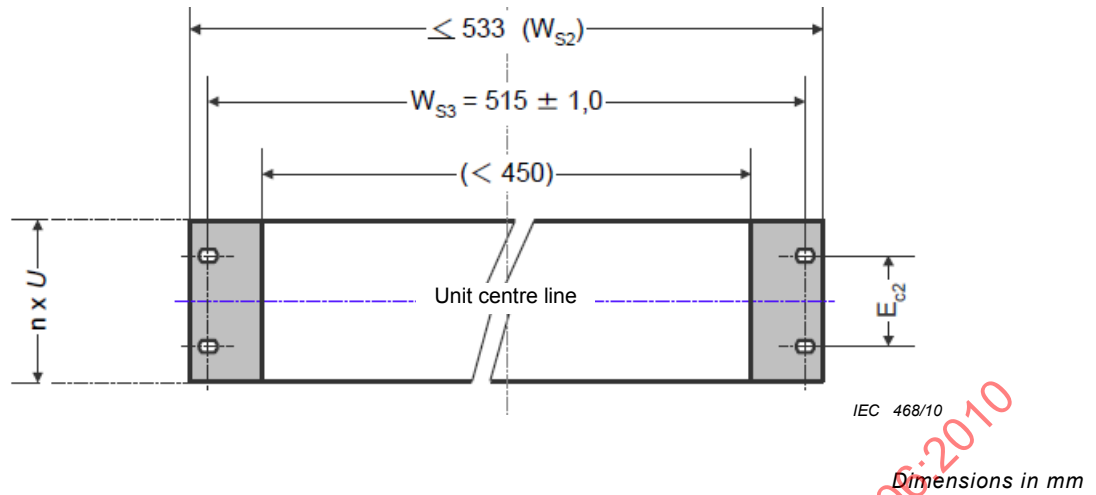
Figure 6 – Dimensions for flanges of 19 in subracks that are applicable for metric cabinets with 515 mm mounting hole dimension
