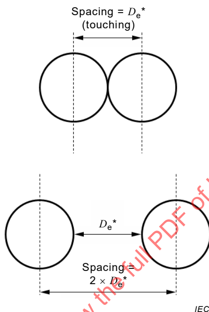
Figure C.1 – Spacing definitions
