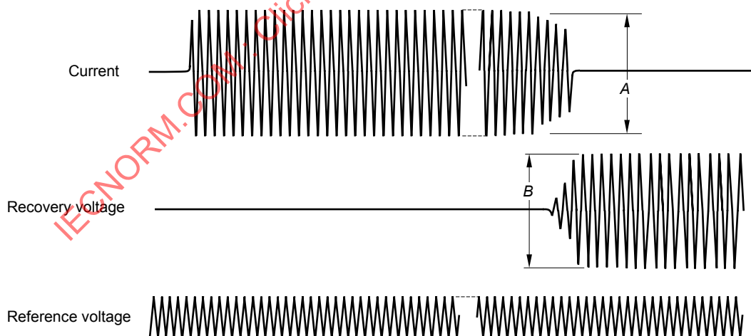
Figure 5b – Test duty 5
