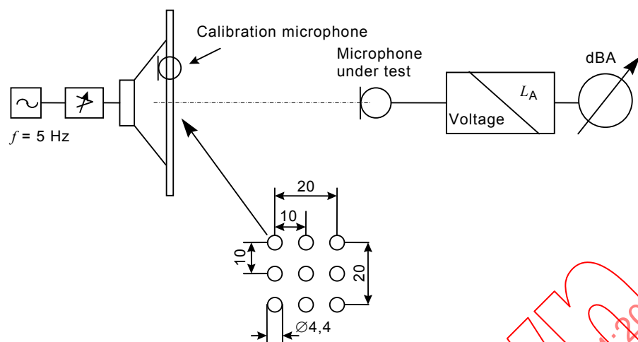
Figure C.1 – Measurement set-up
