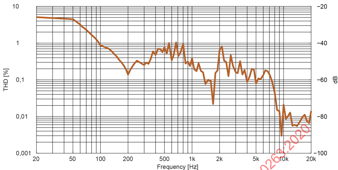
Figure A.8 – Example of total harmonic distortion of a loudspeaker with an aspect ratio of 2,5 decades/decade (50 dB/decade)
