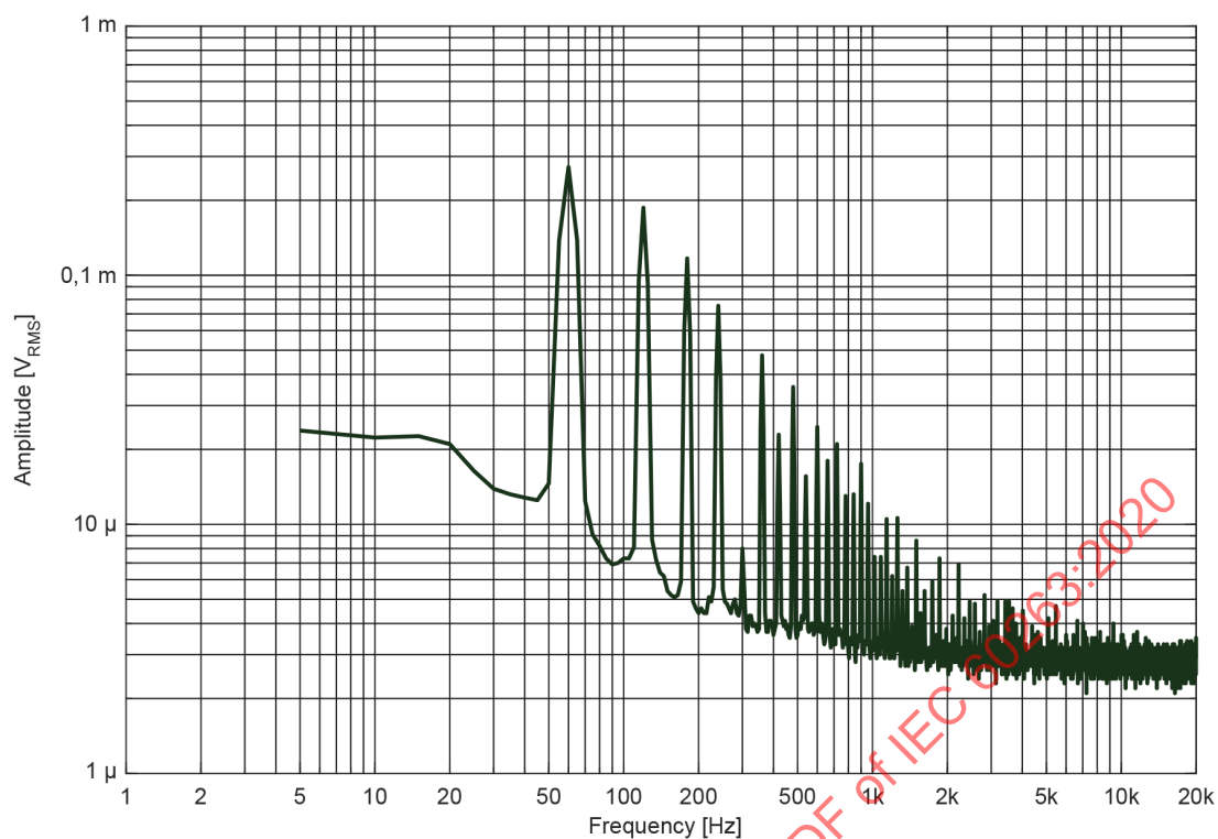
Figure A.6 – Example of amplifier noise with an aspect ratio of 1 decade/decade (20 dB/decade)
