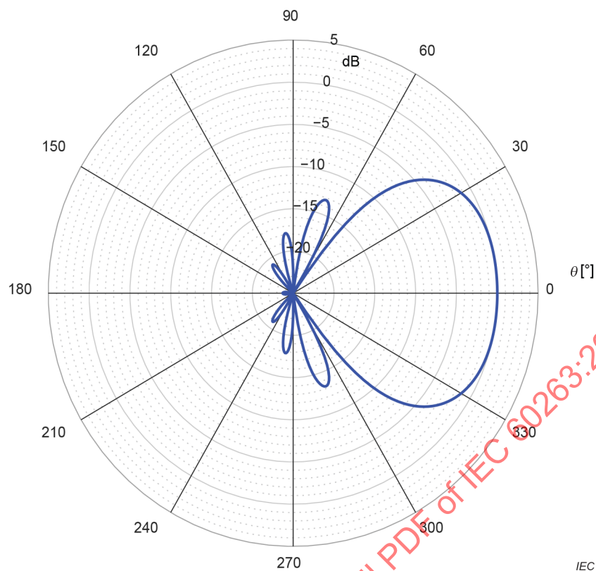
Figure A.10 – Example of a polar diagram of relative level with a range of 30 dB and a reference circle radius of 25 dB, showing the directional response of a highly directional shotgun microphone at 2,5 kHz
