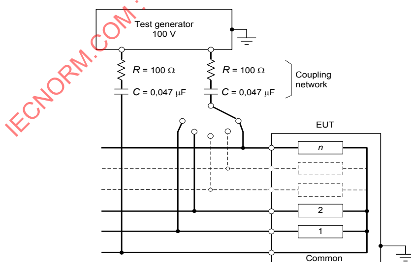
Figure A.1 – Example of Class A differential mode tests
