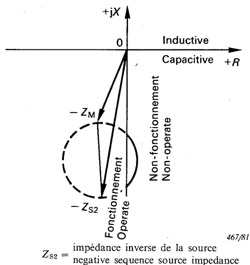
FIG. 1e. — Circular characteristic of phase-to-phase fault, forward direction (left) and reverse direction (right).
