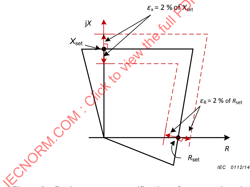
Figure 2 – Basic accuracy specification of an operating characteristic
