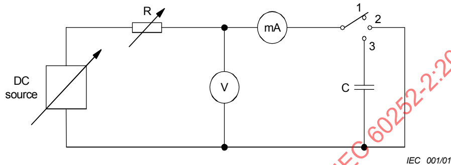
Figure 1 – Test apparatus for d.c. conditioning
