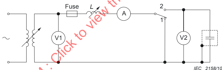
Figure 2 – Test apparatus for a.c. destruction test
