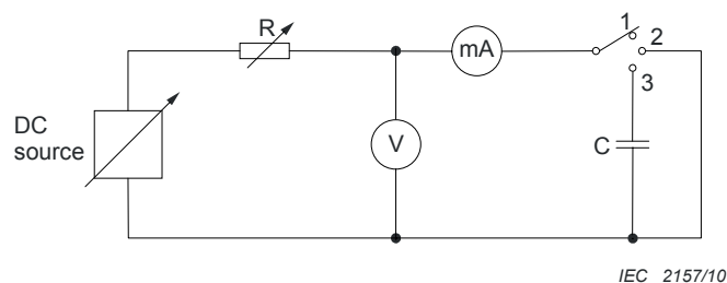
Figure 1 – Test apparatus for d.c. conditioning
