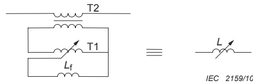
Figure 3 – Arrangement to produce the variable inductor L in Figure 2
