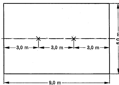
FIG. 1. — Grillage de sol. Wire mesh ground screen.
