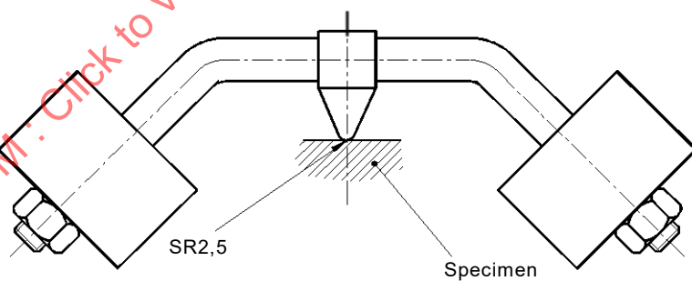
Figure 9 – Pressure apparatus
