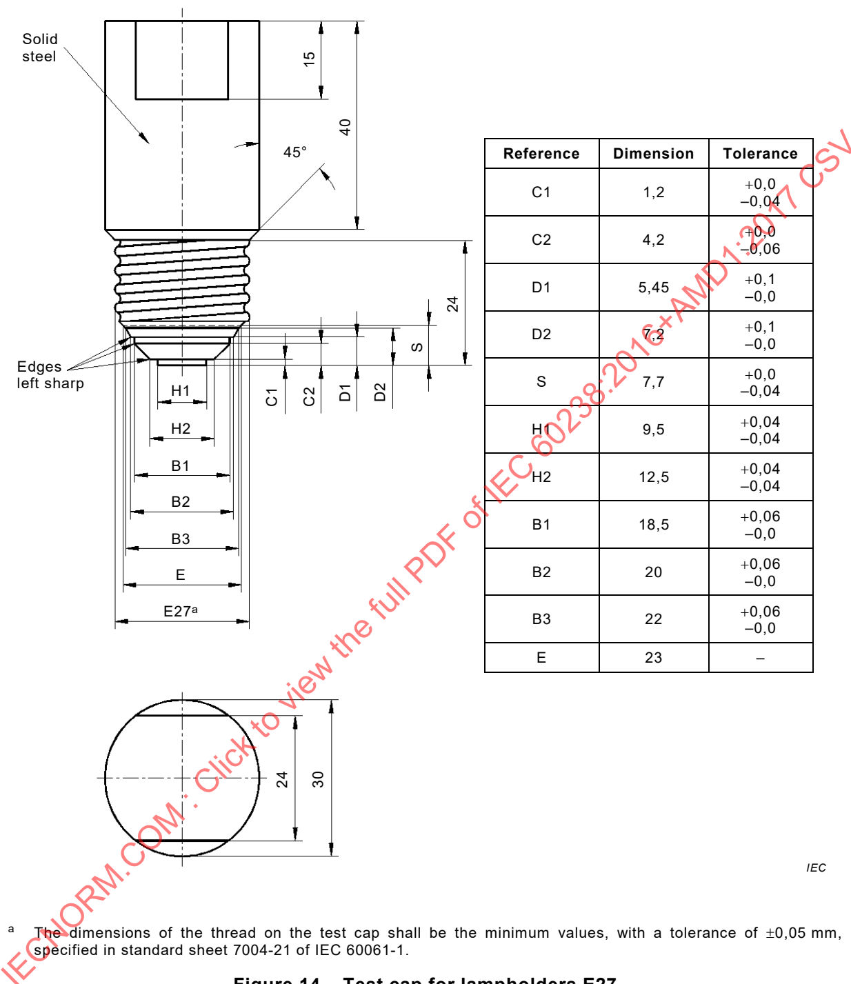
Figure 14 – Test cap for lampholders E27
