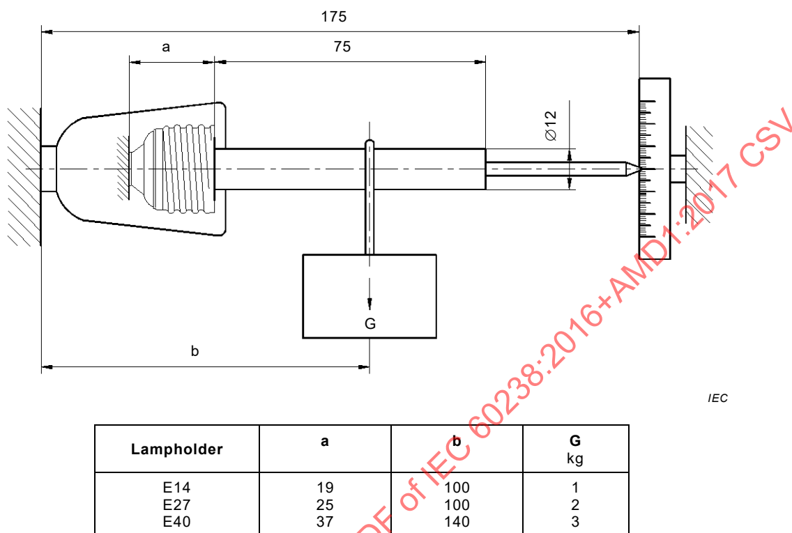
Figure 12 – Bending apparatus
