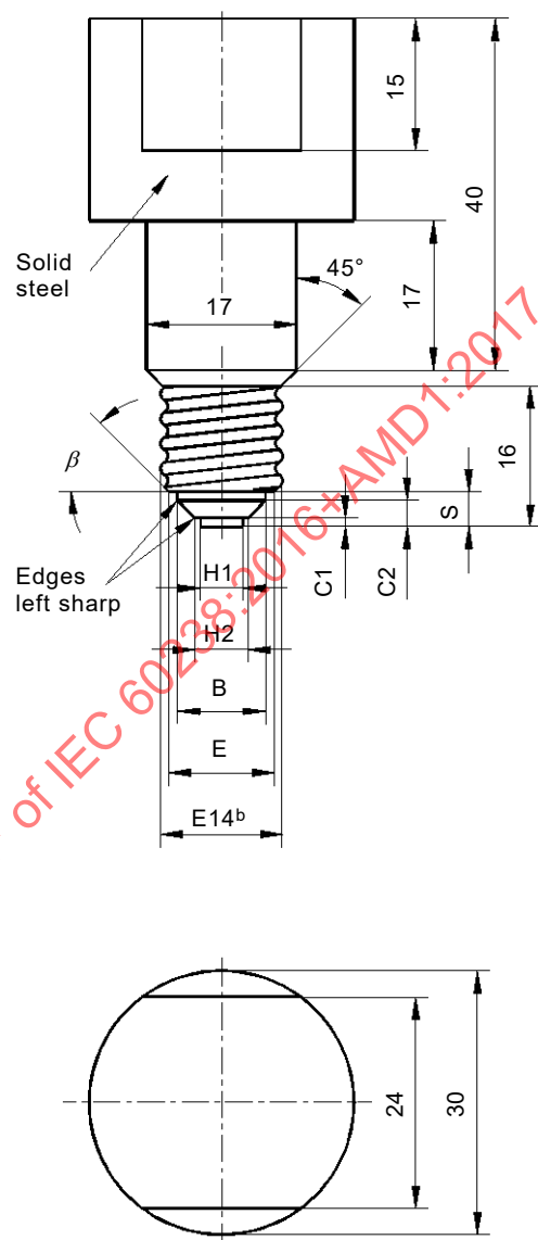
Figure 13b – Test cap B
