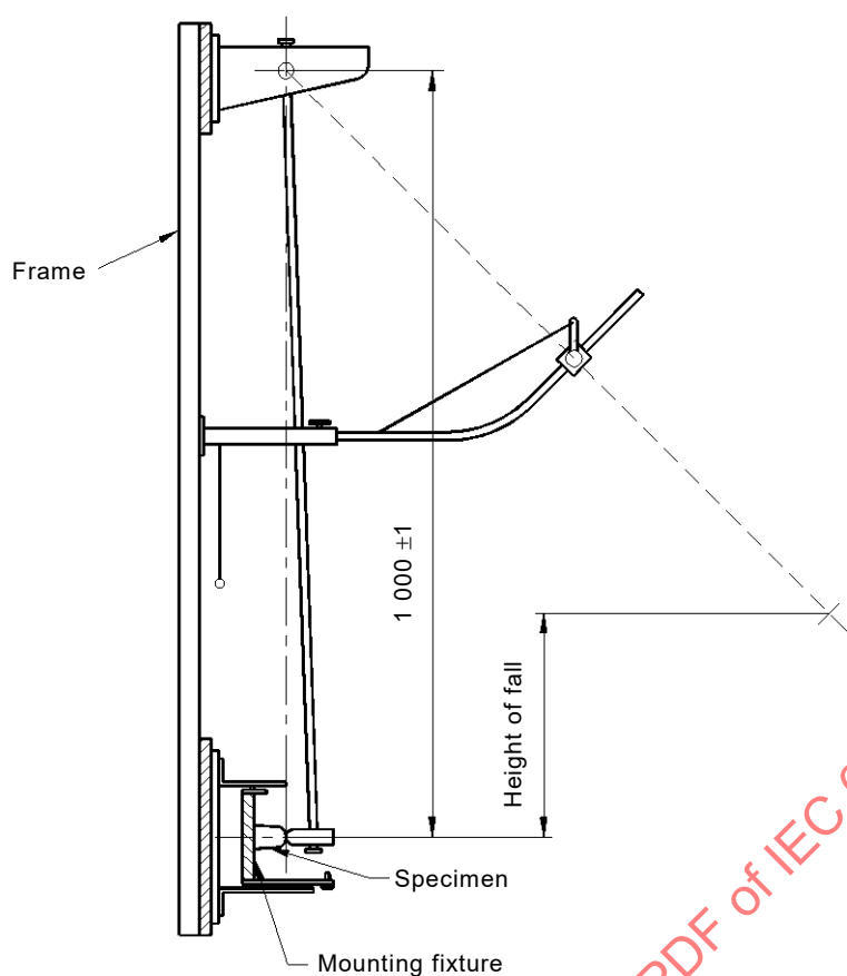
Figure 8a – Impact-test apparatus
