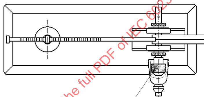
Figure 6 – Torque apparatus
