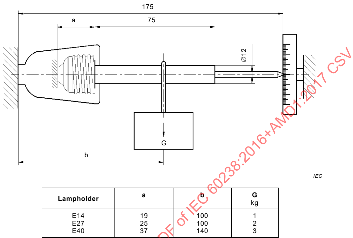
Figure 12 – Bending apparatus
