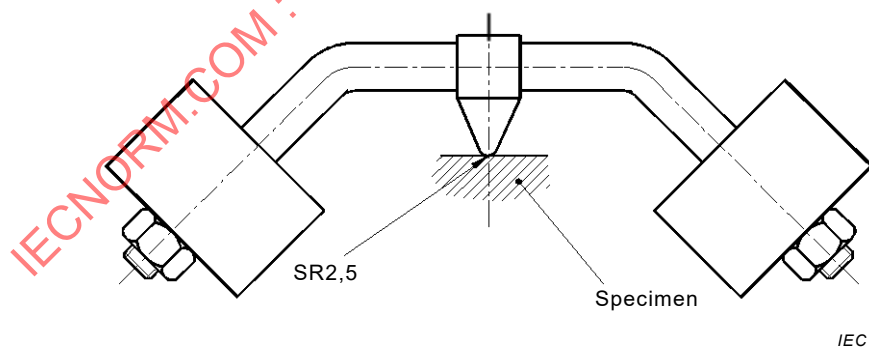
Figure 10 – Ball-pressure test apparatus
