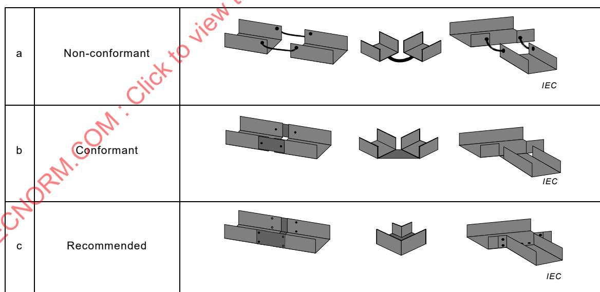
Figure H.5 – Connections between metal cable trays or cable trunking systems
