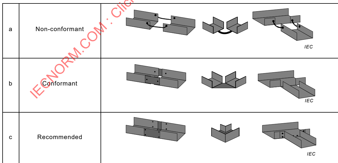
Figure H.5 – Connections between metal cable trays or cable trunking systems
