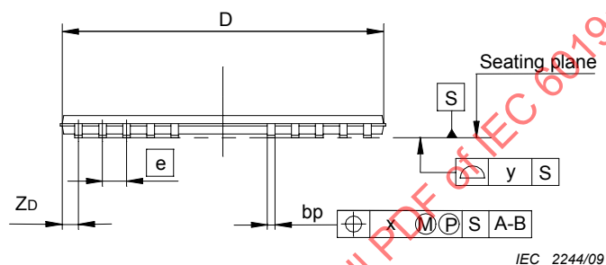
Figure 2b – Side view
