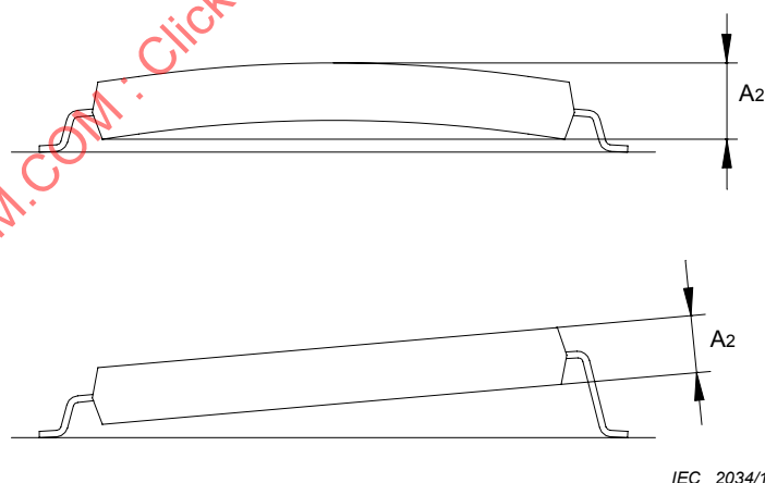
Figure 5 – Body thickness A2
