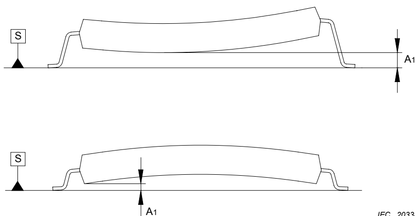
Figure 4 – Stand-off
