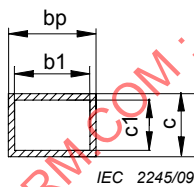
Figure A.3c – Lead section
