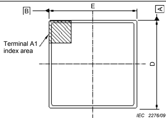
Figure A.15a – Top view
