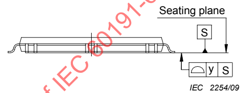
Figure A.7b – Side view
