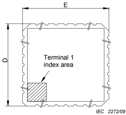
Figure A.13a – Top View
