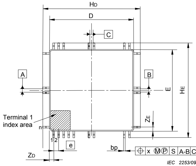
Figure A.7a – Top view
