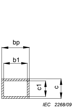
Figure A.11d – Lead section
