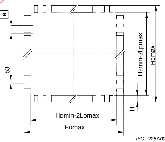
Figure A.8 – Pattern of terminal position areas
