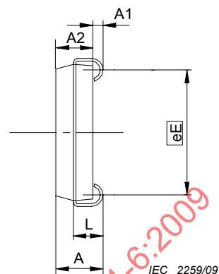
Figure A.9b - Side view
