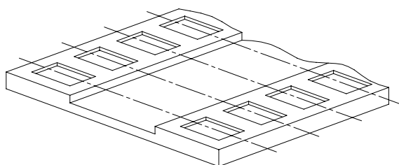
Figure A.1 – Illustrations de la zone de projection de borne
