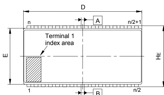
Figure A.9a - Top view
