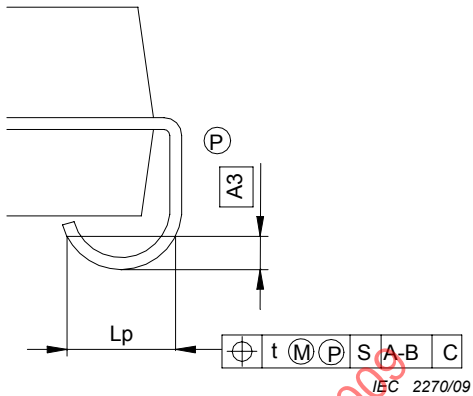
Figure A.11f – Lead side view
