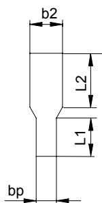
Figure A.9d - Lead shape
