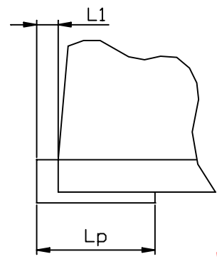
Terminal to be soldered Figure 1e
