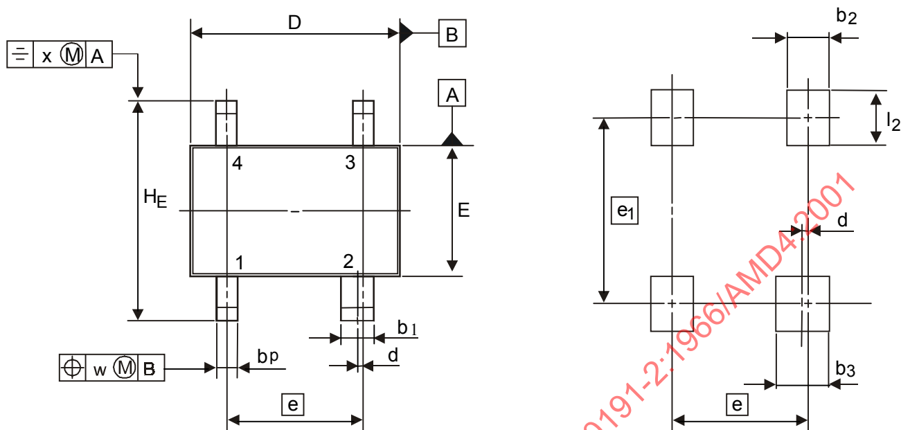
Pattern of terminal land areas
