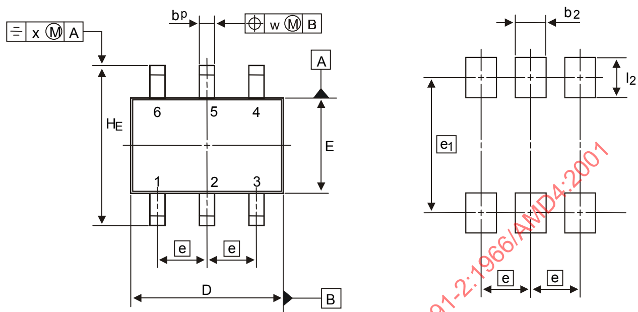
Pattern of terminal land areas
