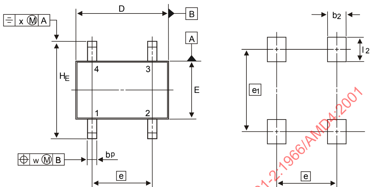
Pattern of terminal land areas
