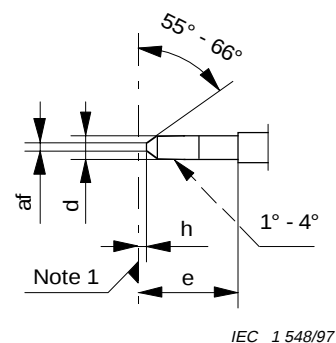
Figure A.4 – Details of pin centre contact
