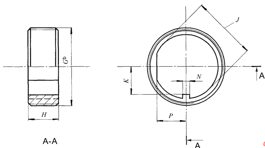
Figure 11 – Bride de type C: 60154 IEC-PCR 220-500
