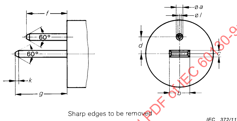
Figure 33 – Gauge for voltage proof and insulation resistance tests of connectors 60130-9 IEC-08
