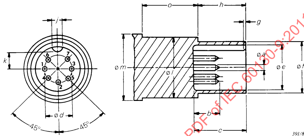
Figure 12 – Fiche 60130-9 IEC-12
