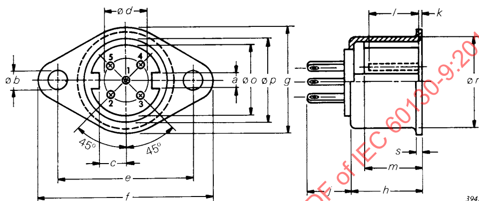
Figure 15 – Embase 60130-9 IEC-15
