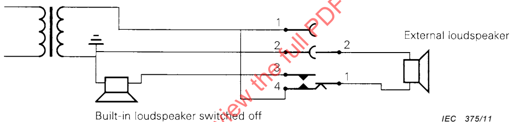
Figure C.2 – Free connector 60130-9 IEC-05 inserted in position B
