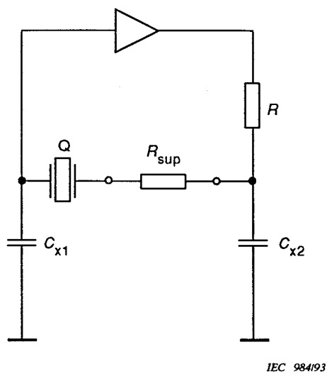
Figure A.2 – Oscillator network with R and R_{sup}
