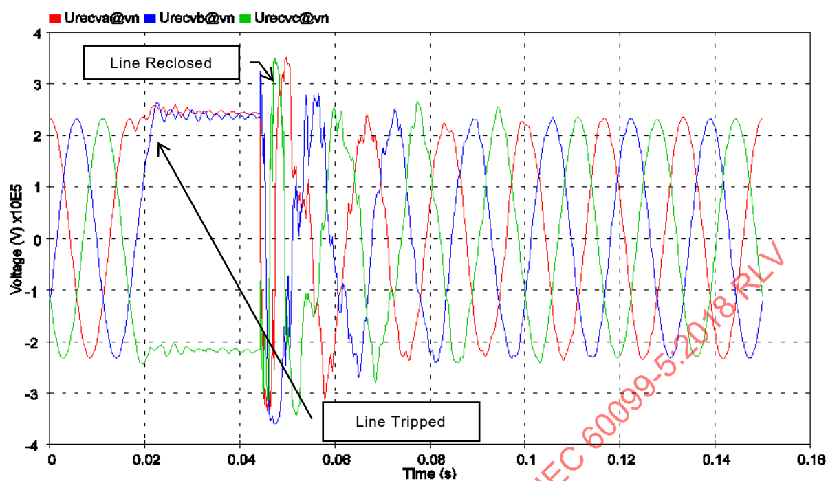
Figure I.17 – U_{ps} for 245 kV system simulation ( V \times 10^5 )
