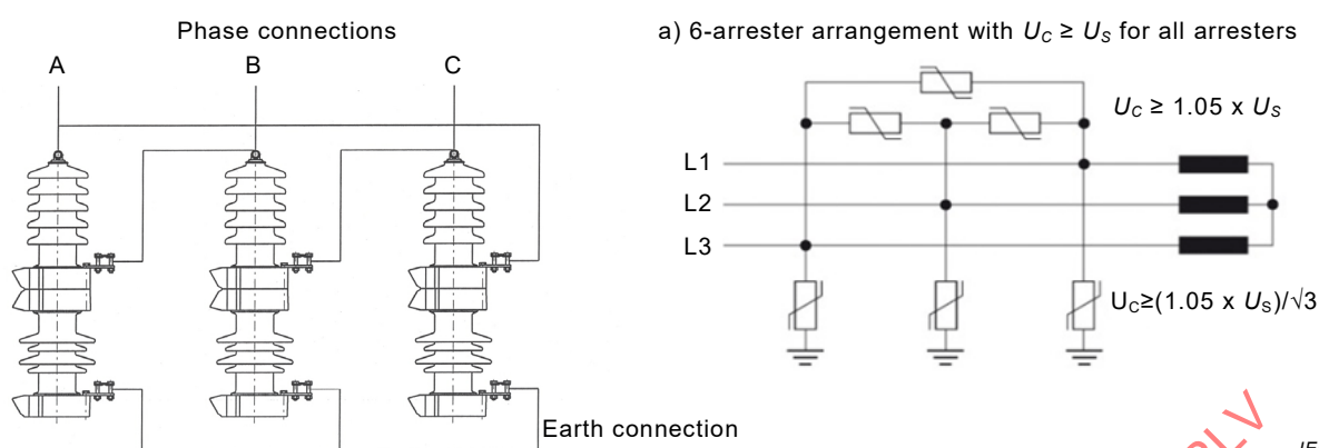
Figure 24a – Six arrester connection
