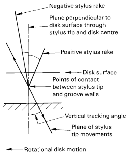
FIG. 1a. - View of groove in direction from stylus tip to disk centre (see Sub-clause 8.1).
