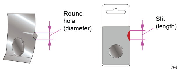
Figure E.5 – Maximum packaging opening
