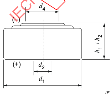
Figure 14 – Dimensional drawing: LR41, LR55, LR54, LR43, LR44
