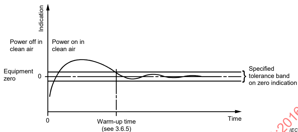
Figure 1 – Warm-up time in clean air (typical)
