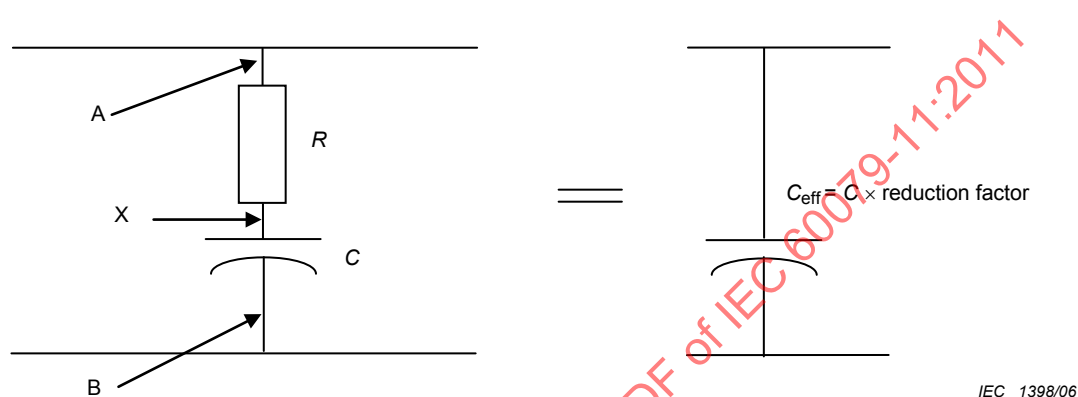
Figure A.9 – Equivalent capacitance
