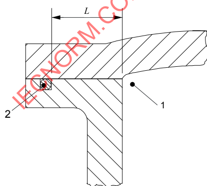
Figure 14 – Illustration of the requirements concerning gaskets – Example 5
