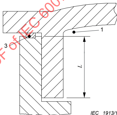
Figure 13 – Illustration of the requirements concerning gaskets – Example 4
