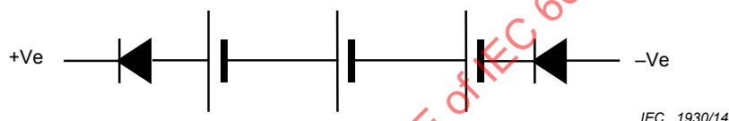
Figure E.2 – Fitting of blocking diodes to meet E.4.3 (third example)
