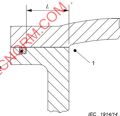
Figure 14 – Illustration of the requirements concerning gaskets – Example 5
