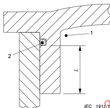
Figure 11 – Illustration of the requirements concerning gaskets – Example 2
