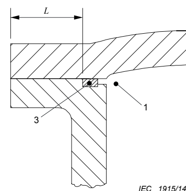
Figure 15 – Illustration of the requirements concerning gaskets – Example 6
