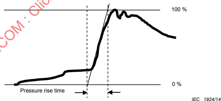
Figure 24 – Example of an irregular shaped waveform
