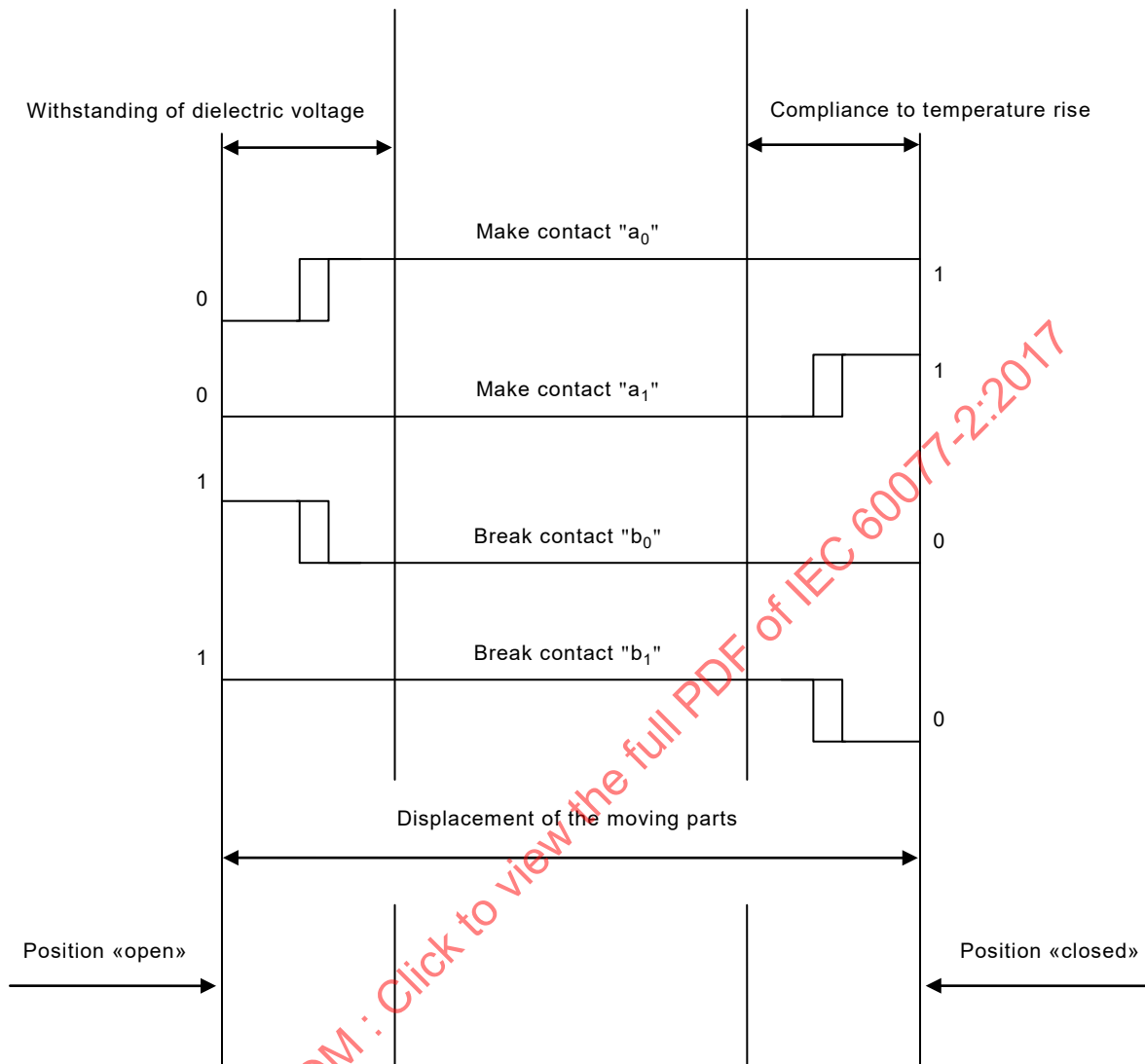
Figure A.1 – Relationship between auxiliary contacts and steady states of switchgear
