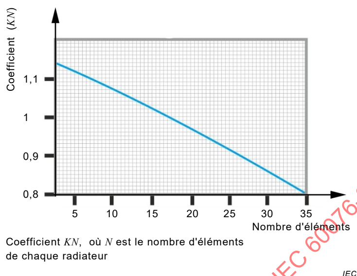
Figure 2 – Coefficient KN
