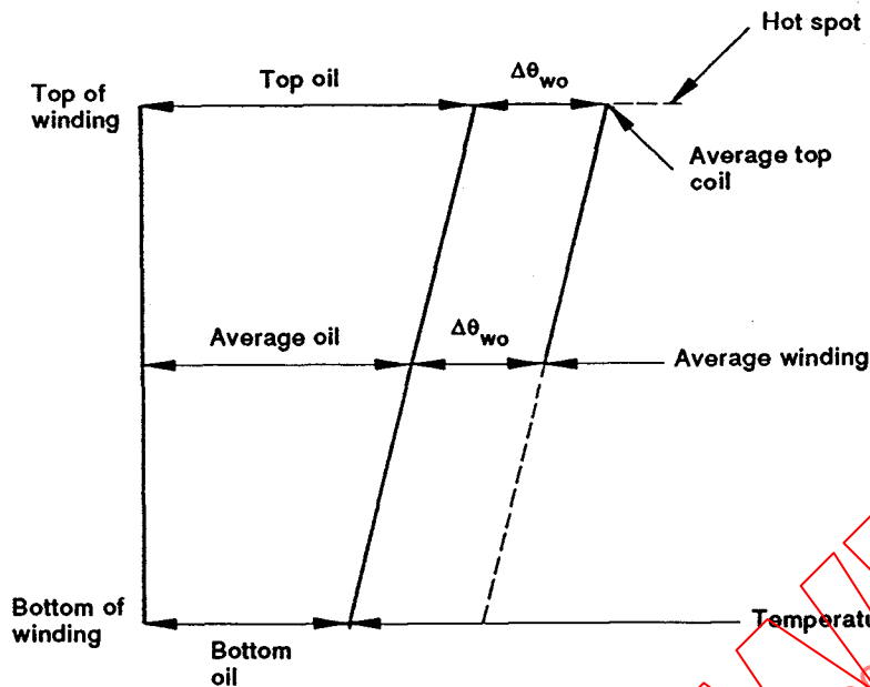
Figure B.1 – Temperature distribution model
