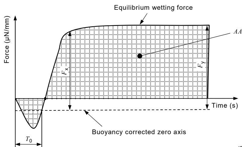
Figure D.1 – Set A wetting curve
