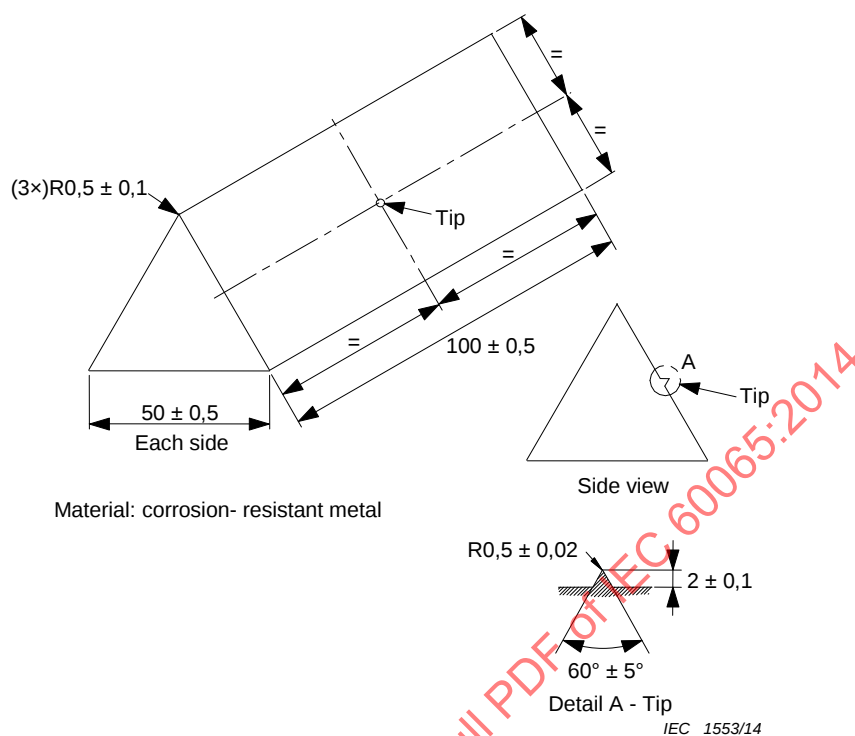
Figure 14 – Mandrel
