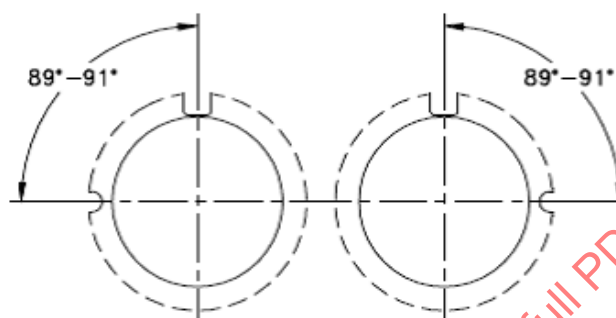
P32d-5 PK32d-5
