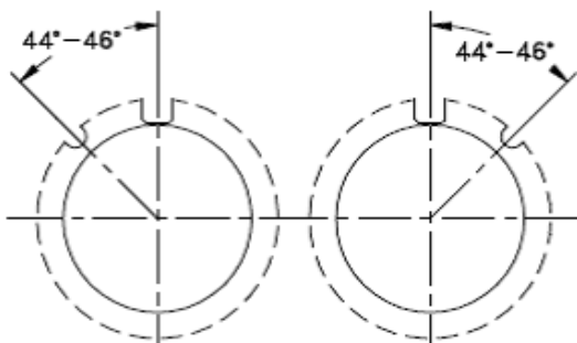
P32d-1 PK32d-1
