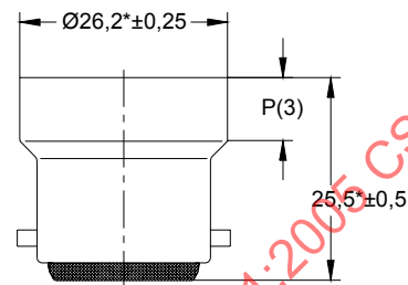
B22d/25x26
