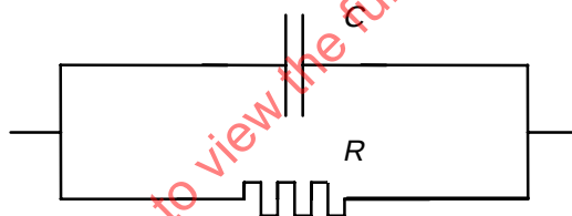
Figure A.2 – Circuit diagram of the capacitive burden for the transient response test
