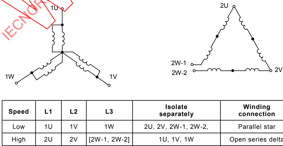
Figure A.15 – Constant-power, seven terminals
