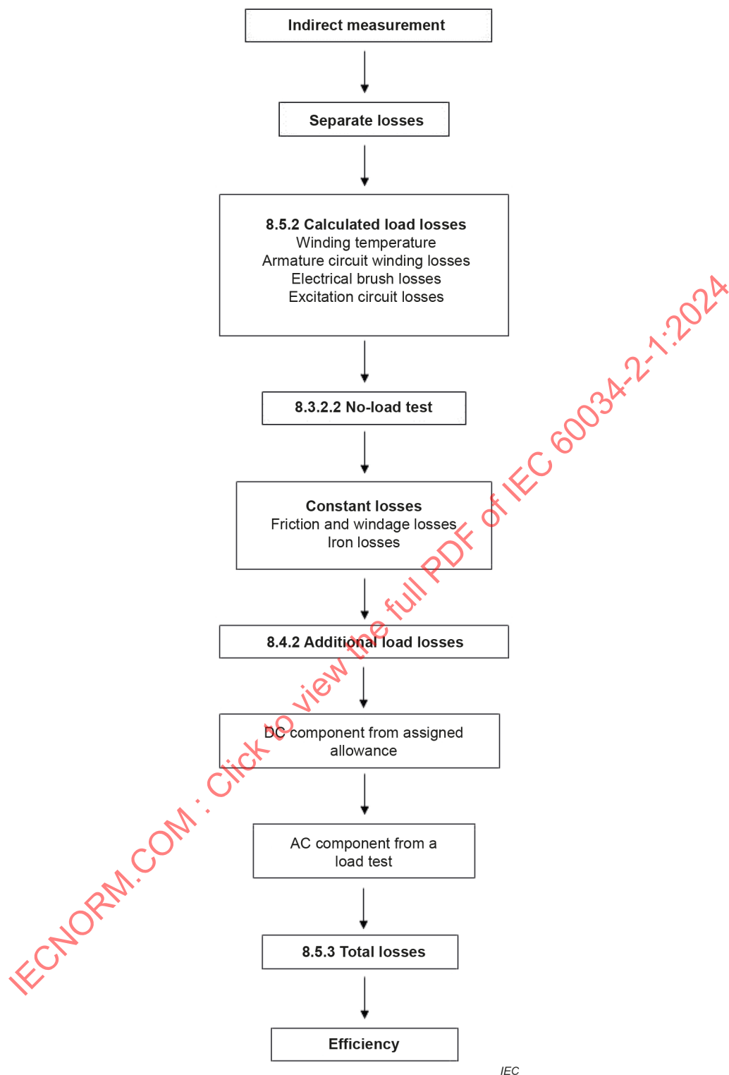
Figure 33 – Efficiency determination according to method 2-1-3D
