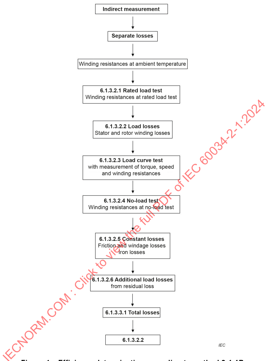
Figure 4 – Efficiency determination according to method 2-1-1B
