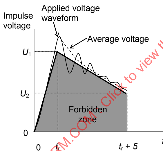
Figure B.1 – Forbidden zone (shaded) for impulse tests
