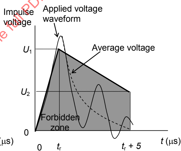
Figure B.1 – Forbidden zone (shaded) for impulse tests
