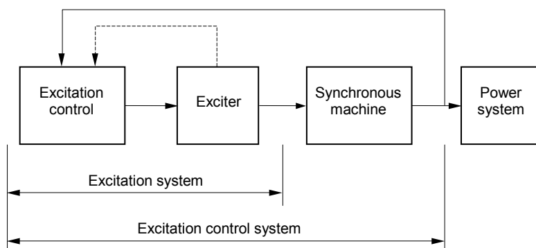
Figure 1 – Block diagram of excitation control system
