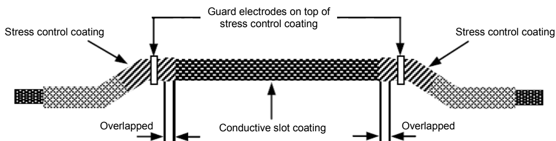
Figure 9 – Application of guard ring electrodes on top of stress control coating
