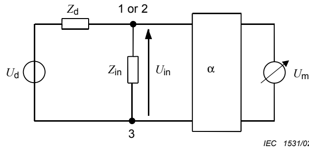
Figure 14 – Basic circuit of the V-AN measurement during the reading of the received voltage U_m (the numbers refer to figure 13)
