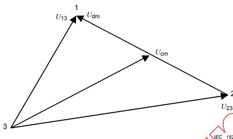
Figure 12 – Relation between the voltages
