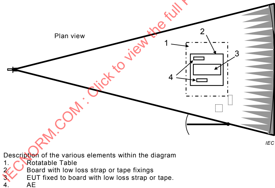
Figure I.3 – Typical EUT mounting for combination of modules being measured
