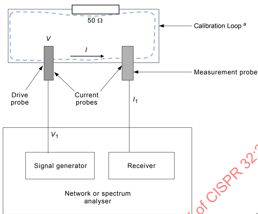
Figure C.6 – Calibration fixture
