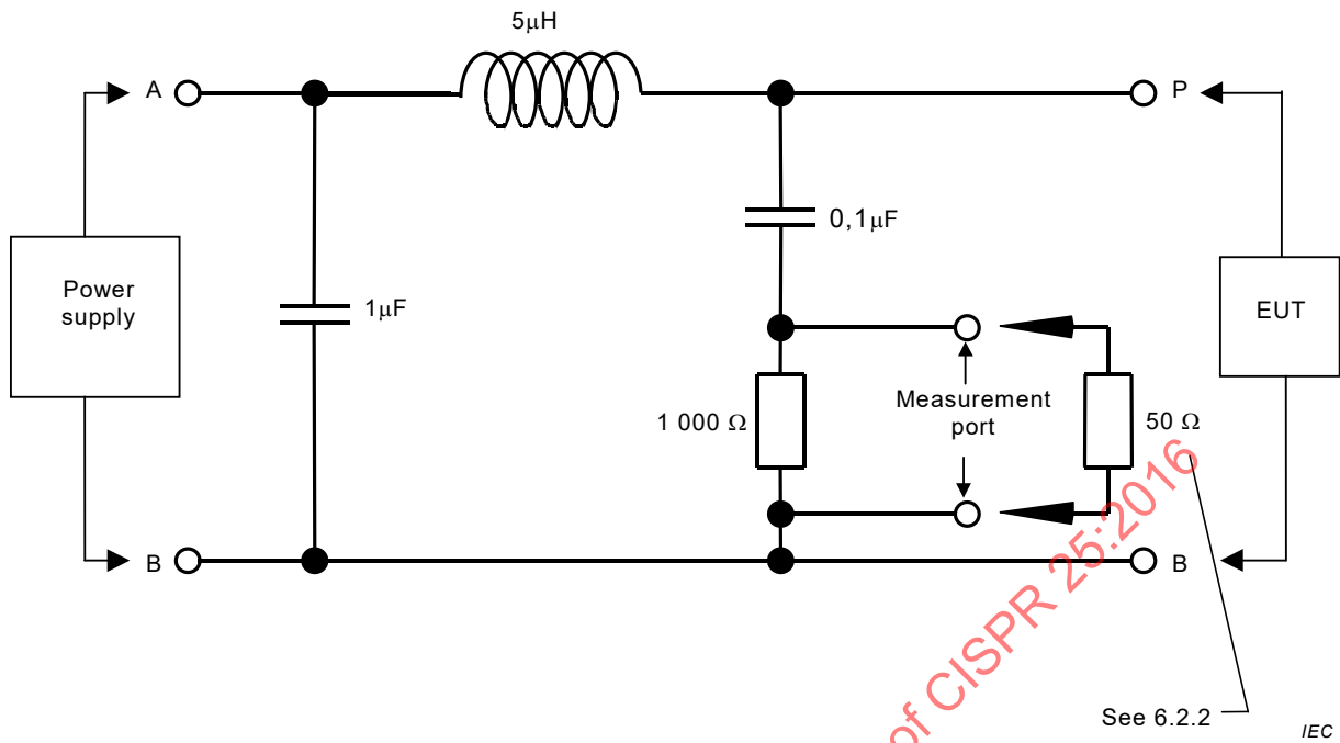
Figure E.1 – Example of 5 \mu\text{H} AN schematic
