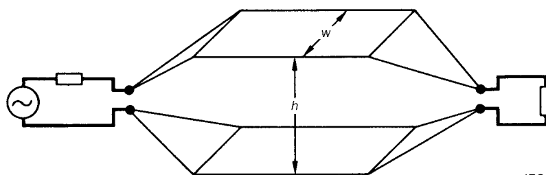
Figure 1 – Open stripline TEM device: basic configuration (see 5.2.2)
