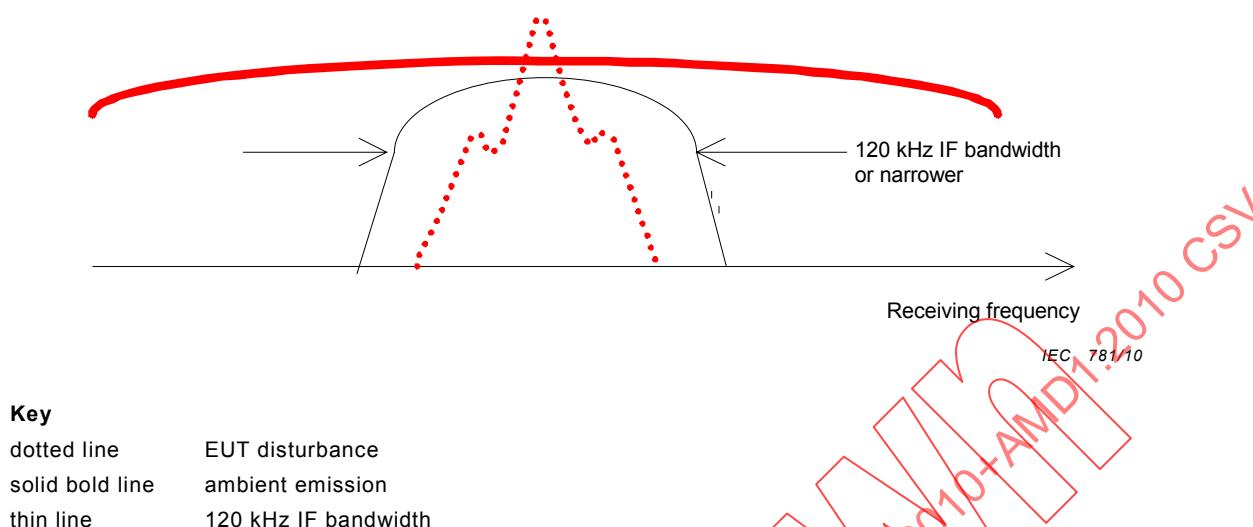
Figure A.9 – Amplitude-modulated EUT disturbance (dotted line)
